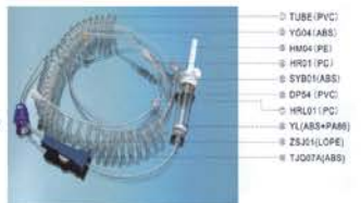
Pressurized Infusion Set AC07022900
