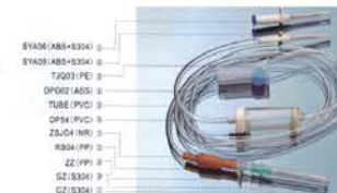
Infusion Set with Double Metal Spike AC07022500
