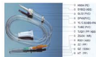
Disposable Infusion Set AC07022100
