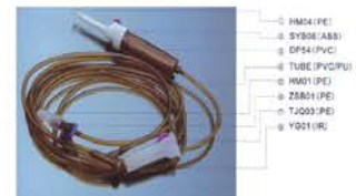
Photophobic Infusion Set AC07022400
