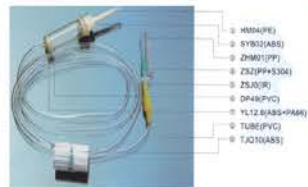
Infusion Set with Precise Flow Regulator AC07022800
