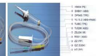
PVC-free Infusion Set AC07022300
